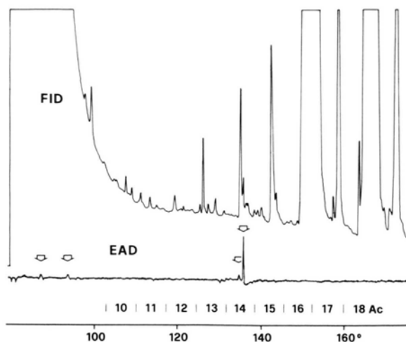
Fig. 1. Gas chromatogram of a Tortrix viridana female wash, recorded with flame ionization (FID) and electroantennographic detection (EAD). Arrows point at EAD peaks reproducible in multiple runs. Elution ranges of straight-chain acetates are indicated. Conditions: Silar 10 C, 22 m \times 0.3 mm glass capillary column. Injection of 1 female equivalent at 70°, after 2 min heated to 90° at 30°/min, then heated at 6°/min to end. The dip in the EAD trace following the main peak is caused by the electronic filter used to compensate for baseline drift.
